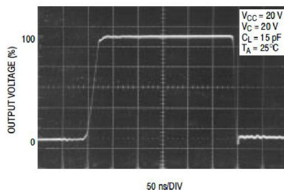
Figure 16. Bottom Drive Output Waveform
