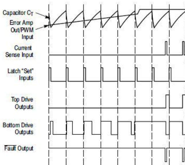
Figure 21. Pulse Width Modulator Timing Diagram
