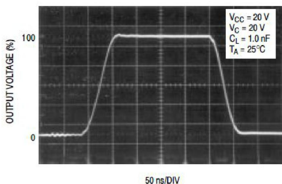
Figure 15. Bottom Drive Output Waveform
