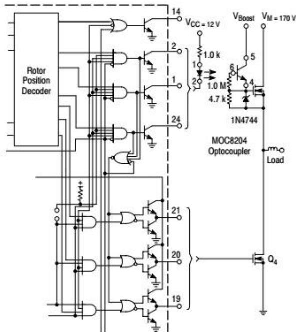
Figure 25. High Voltage Interface with N-Channel Power MOSFETs
