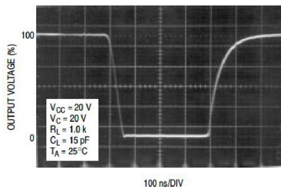
Figure 14. Top Drive Output Waveform
