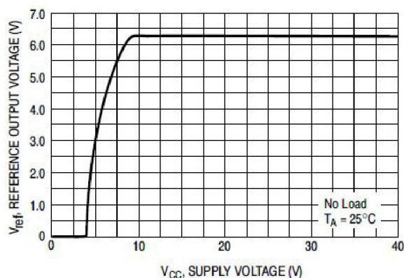
Figure 8. Reference Output Voltage versus Supply Voltage
