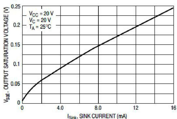
Figure 12. Fault Output Saturation versus Sink Current
