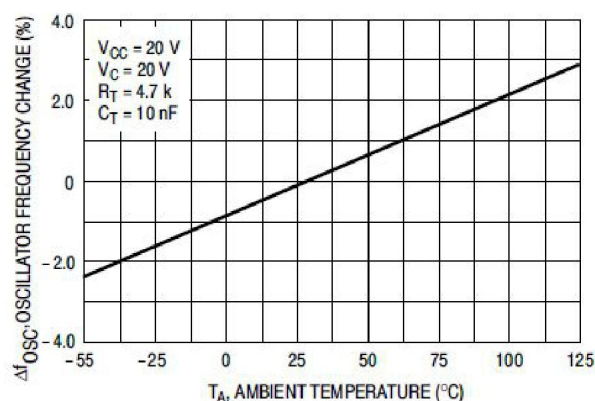
Figure 2. Oscillator Frequency Change versus Temperature
