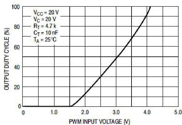
Figure 10. Output Duty Cycle versus PWM Input Voltage
